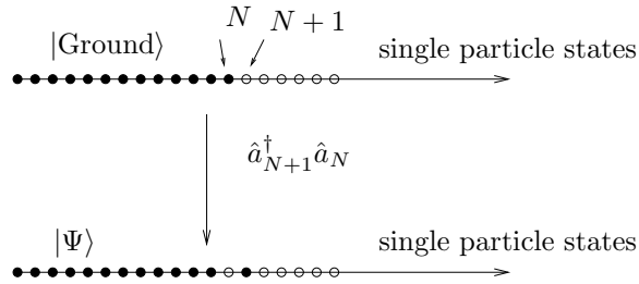
Figure 1.4: An excited (particle-hole) state.
