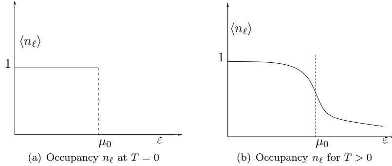
Figure 1.8: The occupation number of eigenstate |\ell\rangle in a free Fermi gas, (a) at T = 0 and (b) for T > 0 . Here, \mu_0 = E_F is the Fermi energy.
