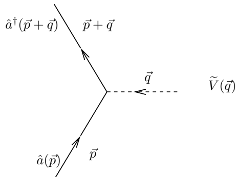
Figure 1.1: One-body scattering.
