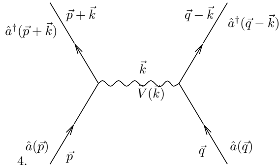
Figure 1.2: Two-body interaction.
