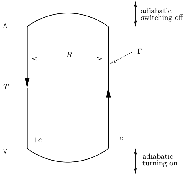
Figure 9.2 The Wilson loop operator can be viewed as representing a pair of quasi-static sources of charge \pm e separated a distance R from each other.
