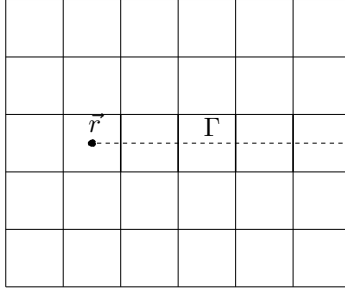
FIG. 10: The dual path \Gamma .
