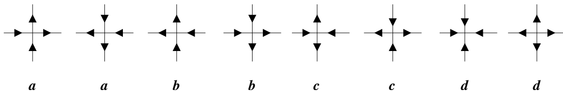
FIG. 3: The eight vertices and their Boltzmann weights
