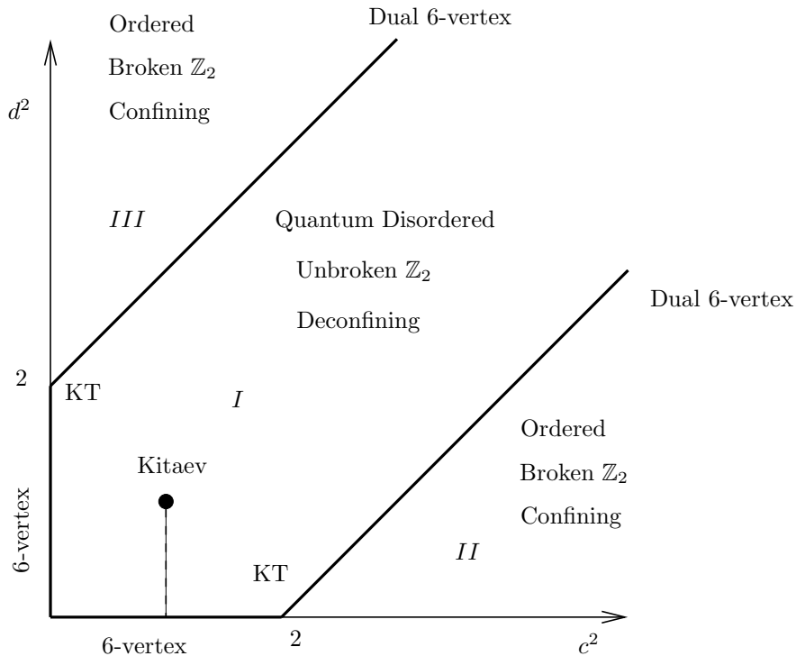
FIG. 5: Phase diagram of the quantum eight-vertex model: phases I and II are separated by a dual 6-vertex transition (same with I and III ); 6-vertex denotes the 6-vertex model critical lines and KT are 2D Kosterlitz-Thouless transitions; the dotted line shows that the Kitaev point is smoothly connected to the critical regime of the eight-vertex model.
