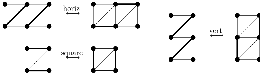
FIG. 1: Dimer flips on the triangular lattice
